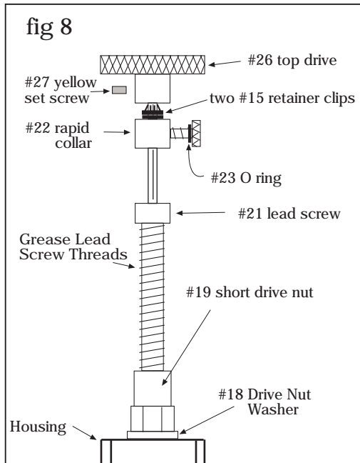
Sub-base or Router Table Insert Plate Installation
